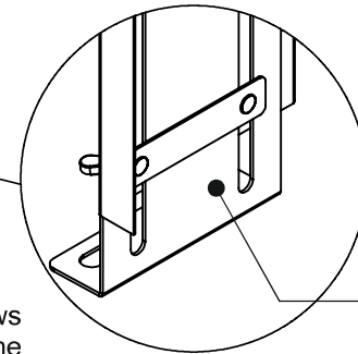
fast and firm clamping of the manifold carrier with wing nuts.
